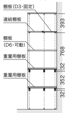
[A-A'断面図]
