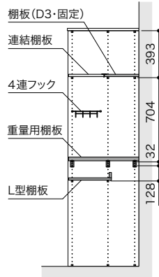
[A-A'断面図]
